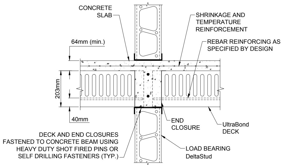
WALL CONNECTION DETAIL
