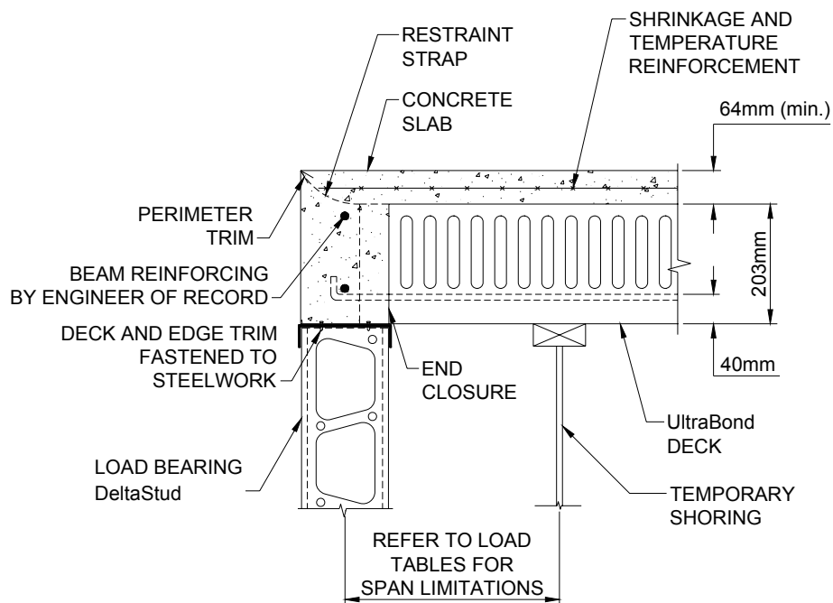
SHORING DETAIL
