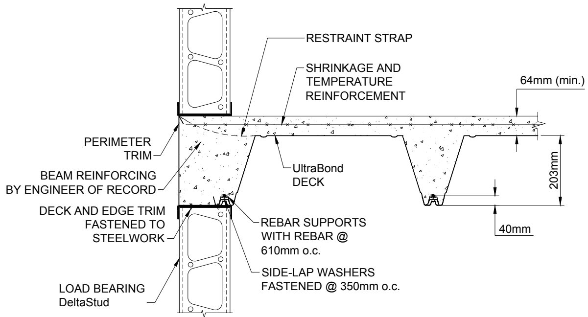
END BEARING DETAIL
